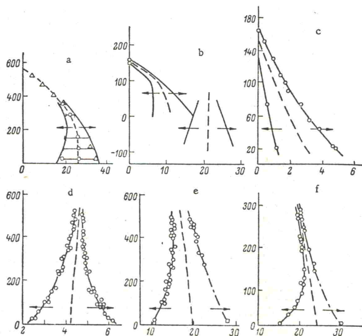
Fig. 1. Hysteresis during phase transformations under pressure: a) Sr [1]; b) \text{AgNO}_3 [1]; c) TlI [2]; d) RbI [3]; e) \text{CdS} [4]; f) InSb [5]. The abscissa axis is pressure (kbars); the ordinate axis is temperature T ( ^{\circ}\text{C} ).
